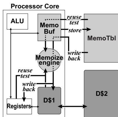
図 1 Structure of Auto-Memoization Processor.
